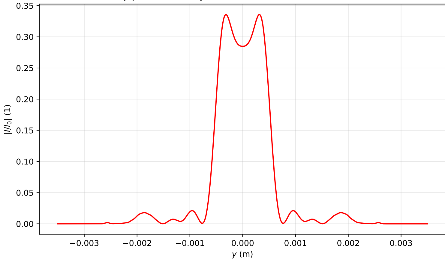
Intensity profile I(x=0, y, z=0.796)/I_0 , P_{in}=3.0P_{cr} , artificial time
